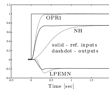
Figure 12.15: Nonlinear simulation results
