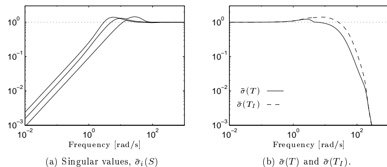
Figure 12.14: Sensitivity and complementary sensitivity functions.
