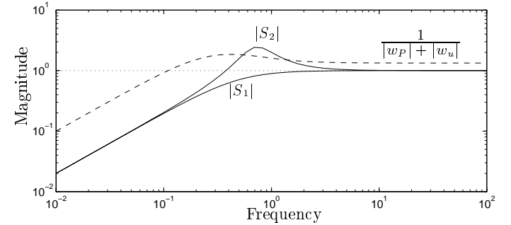
Figure 7.19: Robust performance test
