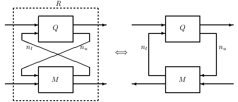
Figure A.8: Star product of Q and M , R = S(Q, M) .
