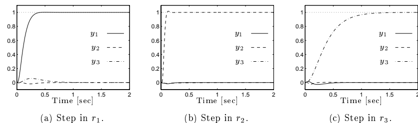
Figure 12.13: Reference step responses.
