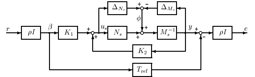
Figure 9.21: Two degrees-of-freedom \mathcal{H}_\infty loop-shaping design problem
