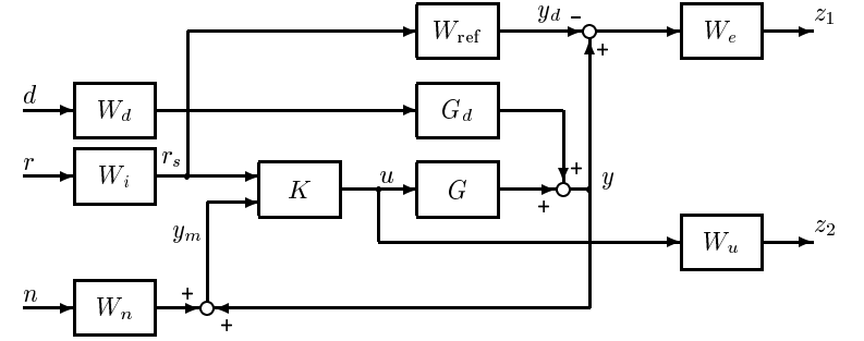
Figure 9.14: A signal-based \mathcal{H}_\infty control problem
