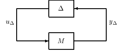
Figure 7.13: M - \Delta structure
