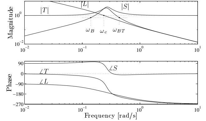
Figure 2.8: Typical Bode magnitude and phase plots of L = GK , S and T . G(s) = \frac{3(-2s+1)}{(5s+1)(10s+1)} , K(s) = 1.136(1 + \frac{1}{12.7s}) (Ziegler-Nichols PI controller).
